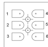
Socket view of screw terminals
