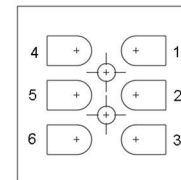
Plug view of screw terminals
