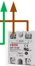
SSR Bed heater
